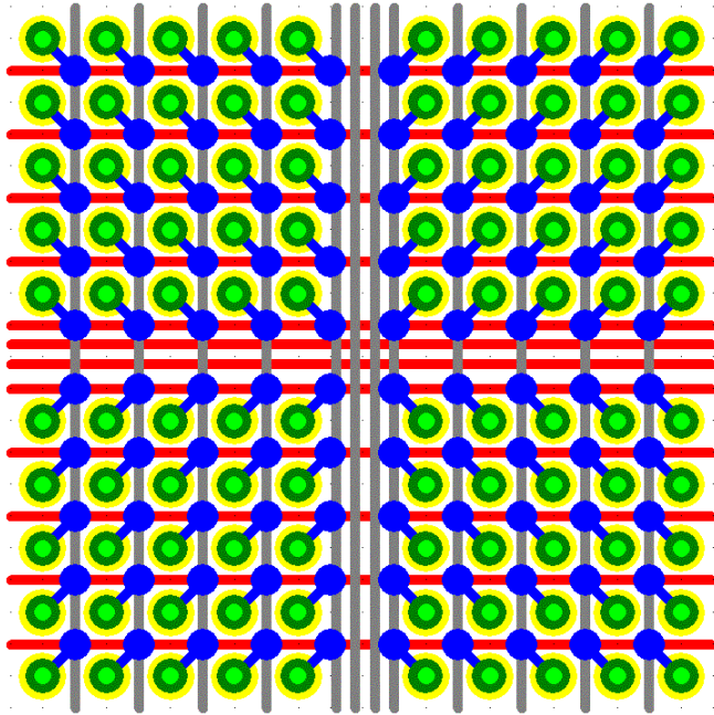
Figure 14: Single Trace Between Vias
