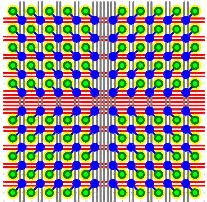
Figure 15: Double Trace Between Vias
