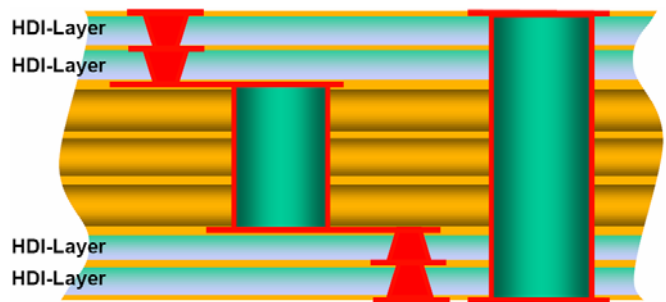
Figure 6: Stacked Micro Vias
