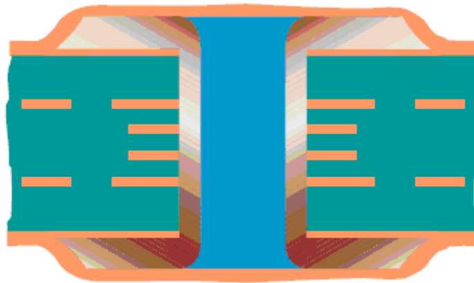
Figure 10: Plated, Filled and Capped BGA Land
