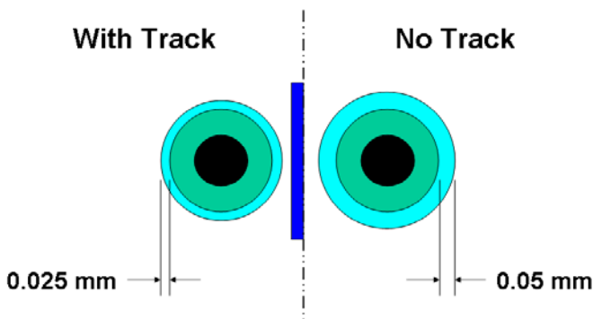
Figure 3: 0.4 Pitch BGA Solder Mask Clearance
