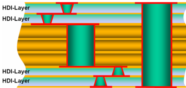
Figure 5: Staggered Micro Vias
