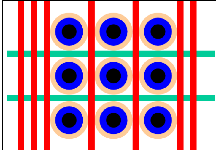
Figure 1: BGA Using Via-in-Land Technology
