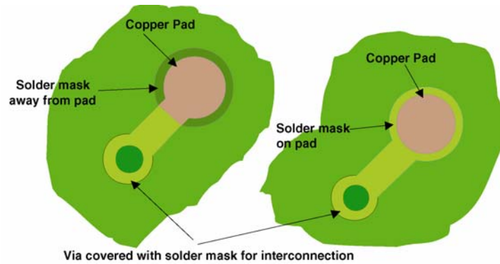
Figure 11: Solder Lands for BGA Components
