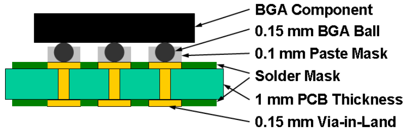
Figure 9: Non-Collapsing 0.5 mm pitch BGA
