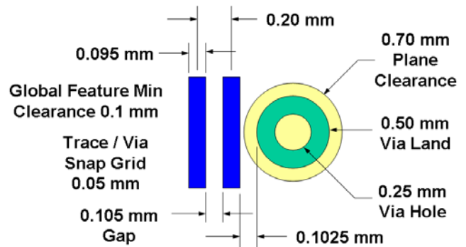
Figure 17: Controlled Impedance Single Ended Traces for 1 mm pitch BGA
