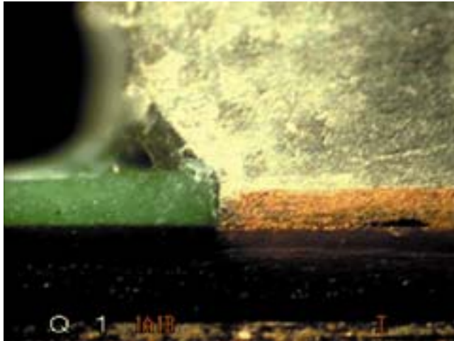
Figure 13: Cross-sectional view of land with solder ball joint illustrating the solder wetting down the edge of the land with solder mask relief away from the land edge
