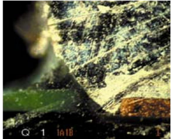
Figure 13: Cross-sectional view of land with solder ball joint illustrating the solder wetting down the edge of the land with solder mask relief away from the land edge
