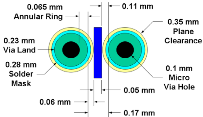
Figure 2: 0.4 Pitch BGA using Micro Via Technology
