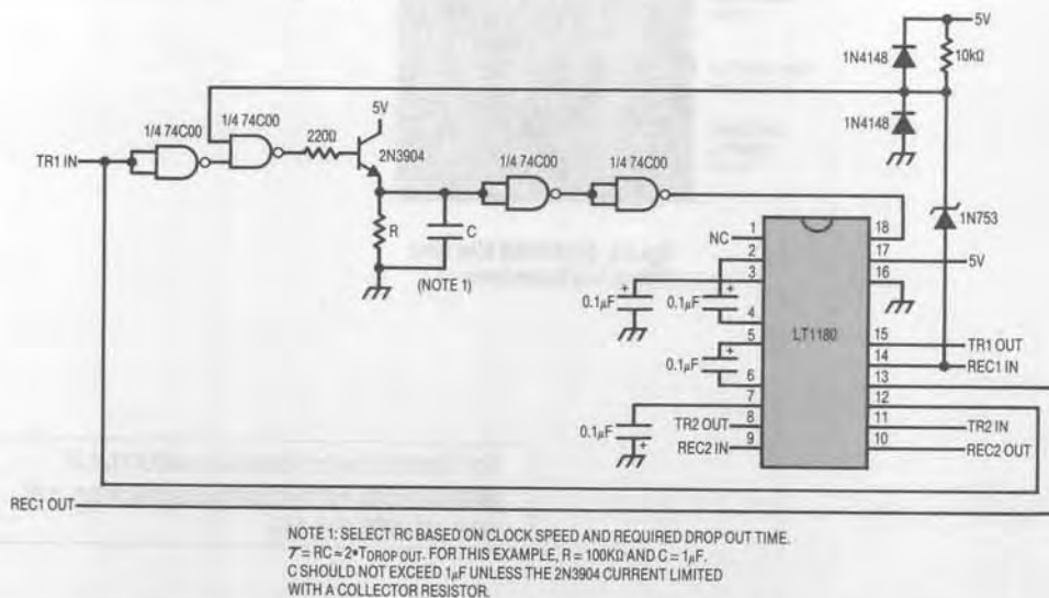
Figure 1. Fast Turn-On Transceiver with Automatic SHUTDOWN Control
