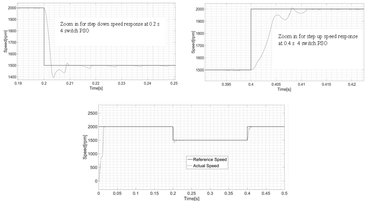
Figure 12. Set point tracking for PSO based tuning PI speed controller of BLDC motor drive fed by four switch inverters
