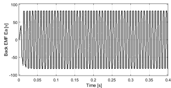
Figure 9. Back EMF response of PSO based tuned PI controller of BLDC motor drive fed by four switch inverters
