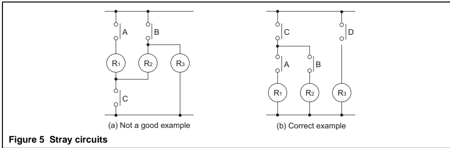
Figure 5 Stray circuits
