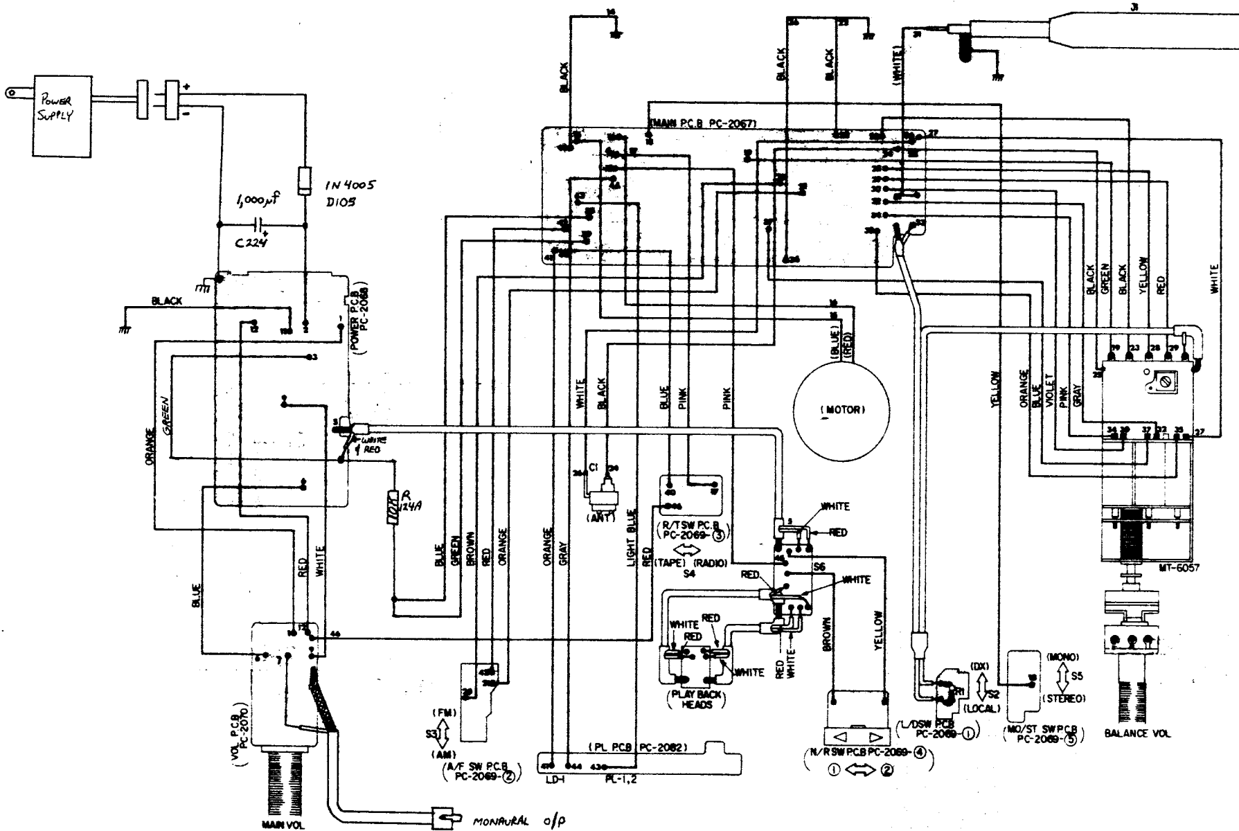
Fig. 5 WIRING DIAGRAM SRX 153 SP
