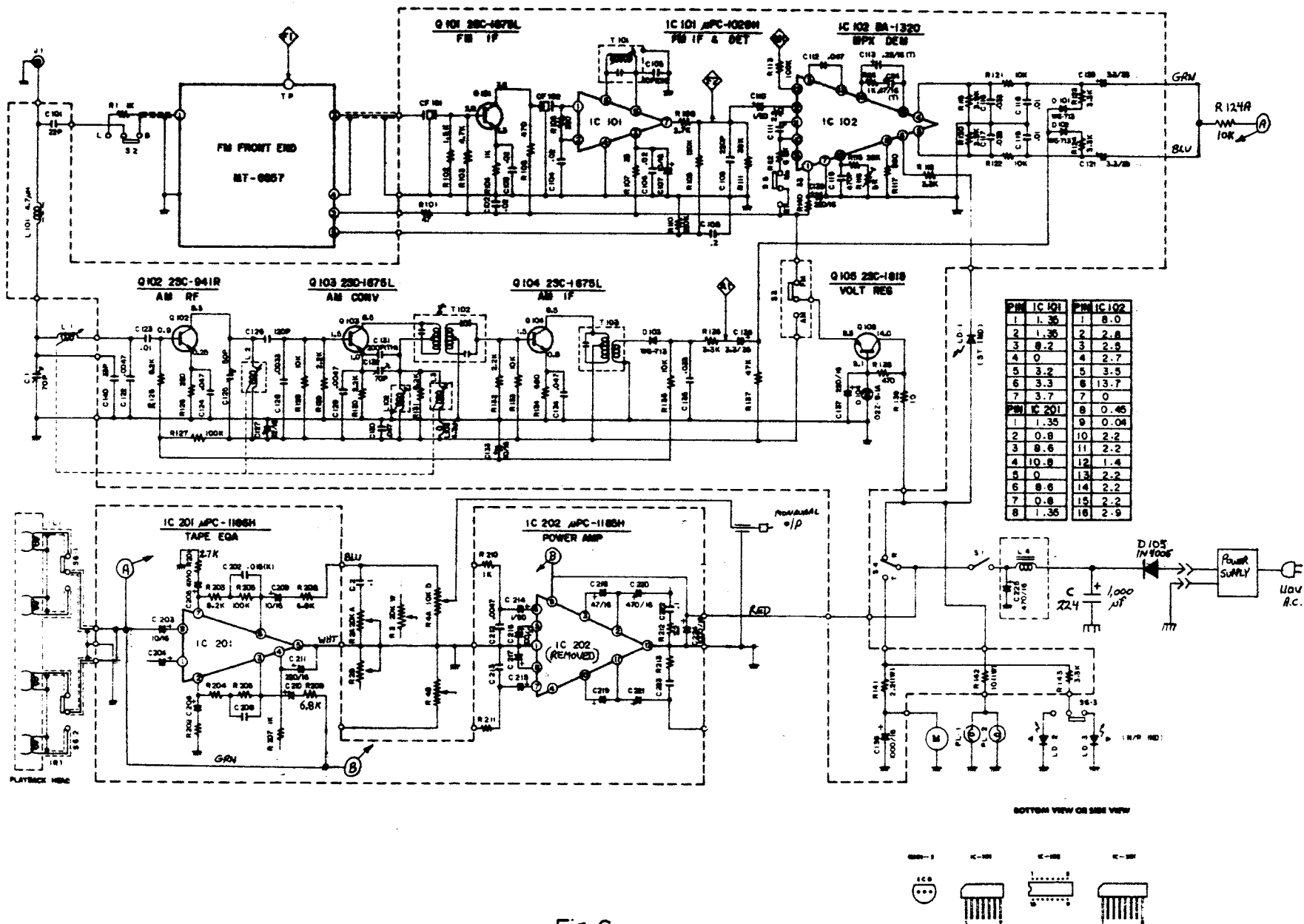
Fig. 6 SCHEMATIC DIAGRAM SRX 153 SP
