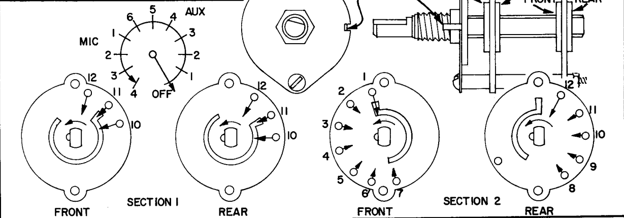
SW (MODEL 19A105) - 680-432 (SWITCH CONTACTS VIEWED FROM REAR - SHOWN IN "OFF" POSITION)
