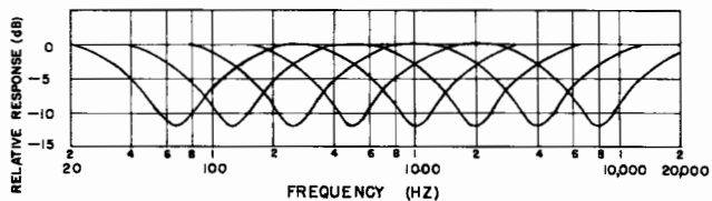
FIGURE D2—EACH FILTER AT MAXIMUM ATTENUATION
