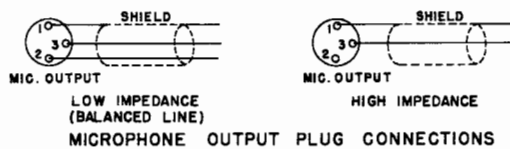
MICROPHONE CONNECTIONS FIGURE B
