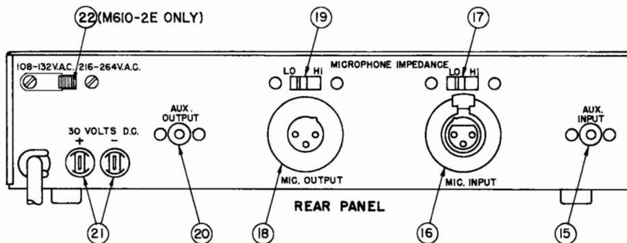
CONTROLS AND CONNECTORS FIGURE C
