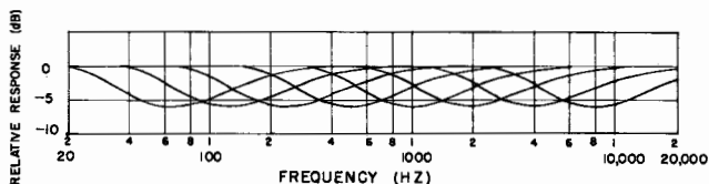
FIGURE D1—EACH FILTER AT 6 dB ATTENUATION
