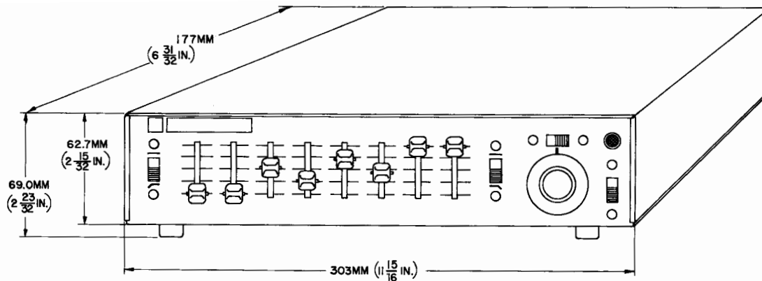
OVERALL DIMENSIONS FIGURE A
