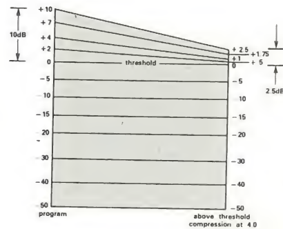
Fig. 7 — Above Threshold Compression Above threshold compression has no effect on low level signals. When signal level reaches the adjustable threshold, the dynamic content of the music is decreased but only above that threshold. Higher compression ratios may be used in above threshold compression than in linear compression; however, all ratios are available. This is known as limiting if the compression ratio is 10:1 or higher.
