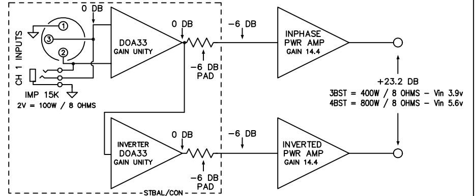
ST REG - BALANCED INPUT - BRIDGED MODE
