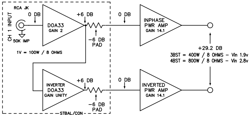
ST PRO - UNBALANCED INPUT - BRIDGED MODE
