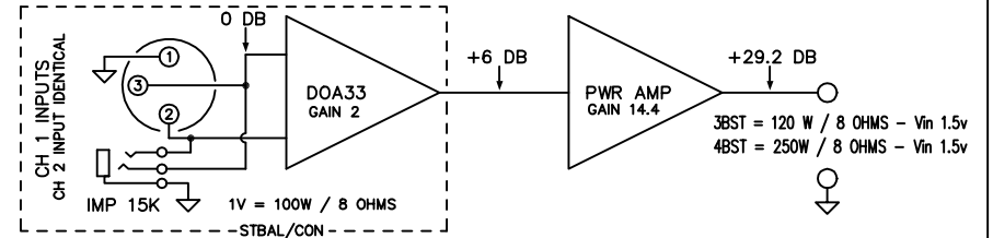
ST PRO - BALANCED INPUT - BRIDGED MODE
