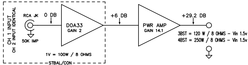
ST PRO - UNBALANCED INPUT - BRIDGED MODE
