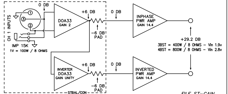
ST PRO - BALANCED INPUT - BRIDGED MODE
