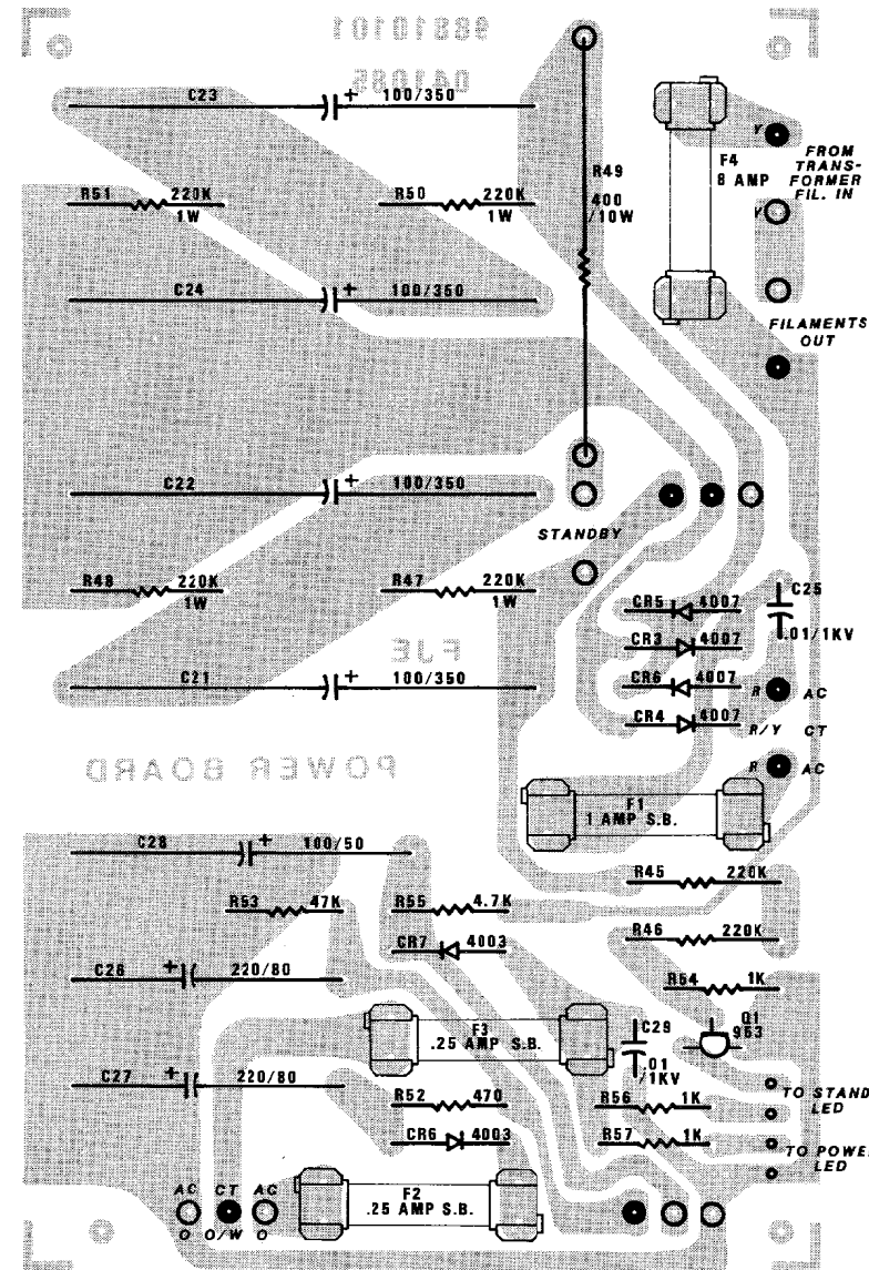
BUTCHER POWER BD.
