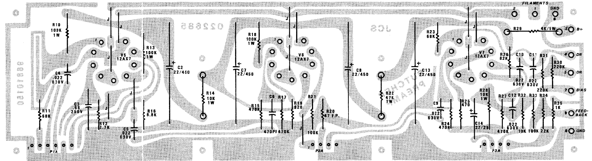
BUTCHER PREAMP BD.
