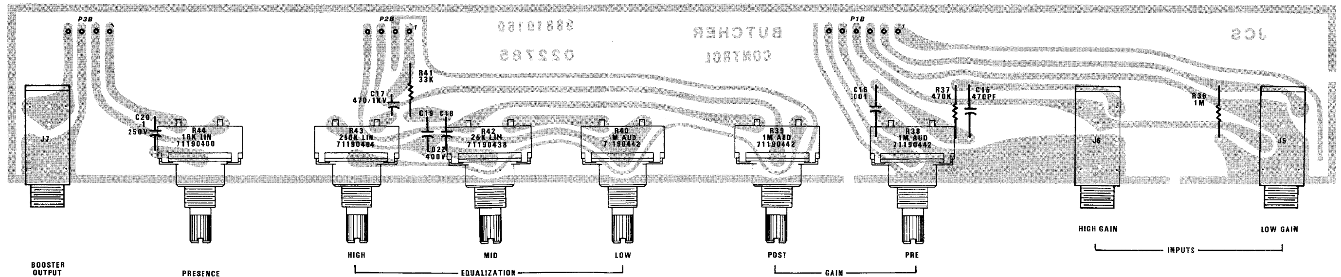
BUTCHER CONTROL BD.
