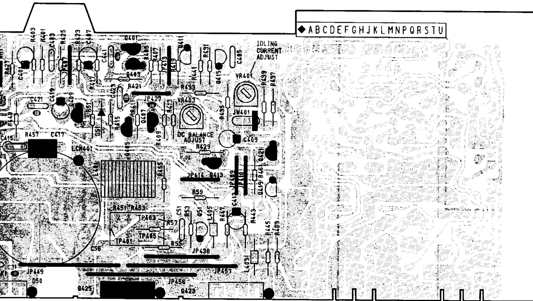
PCB 106 BIAS 2 P.C. BOARD
