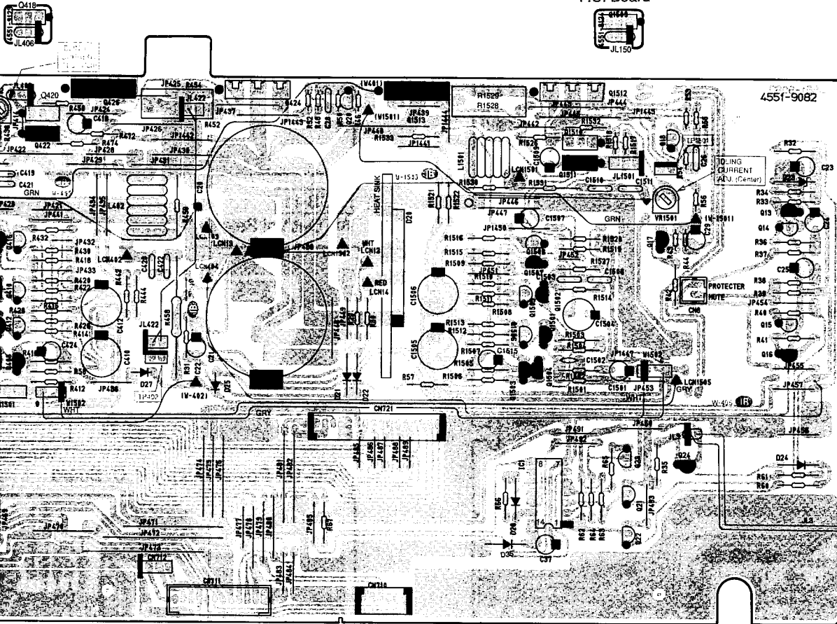
Main R-ch Bias P.C. Board
