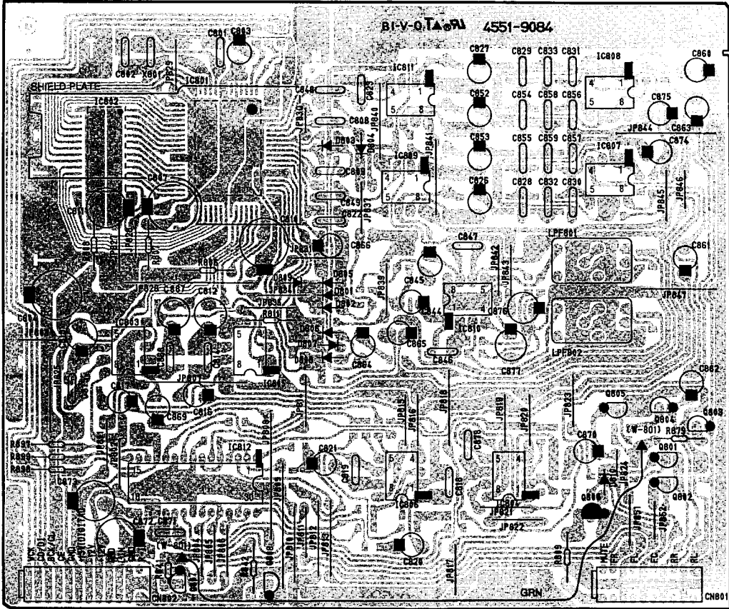
PCB-23 DSP P. C. Board (Parts Side)
