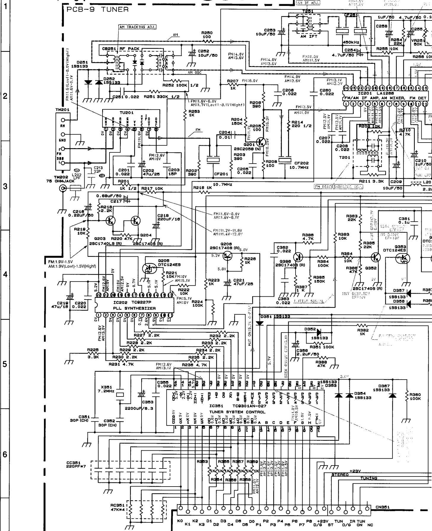
SCHEMATIC DIAGRAM(12)
