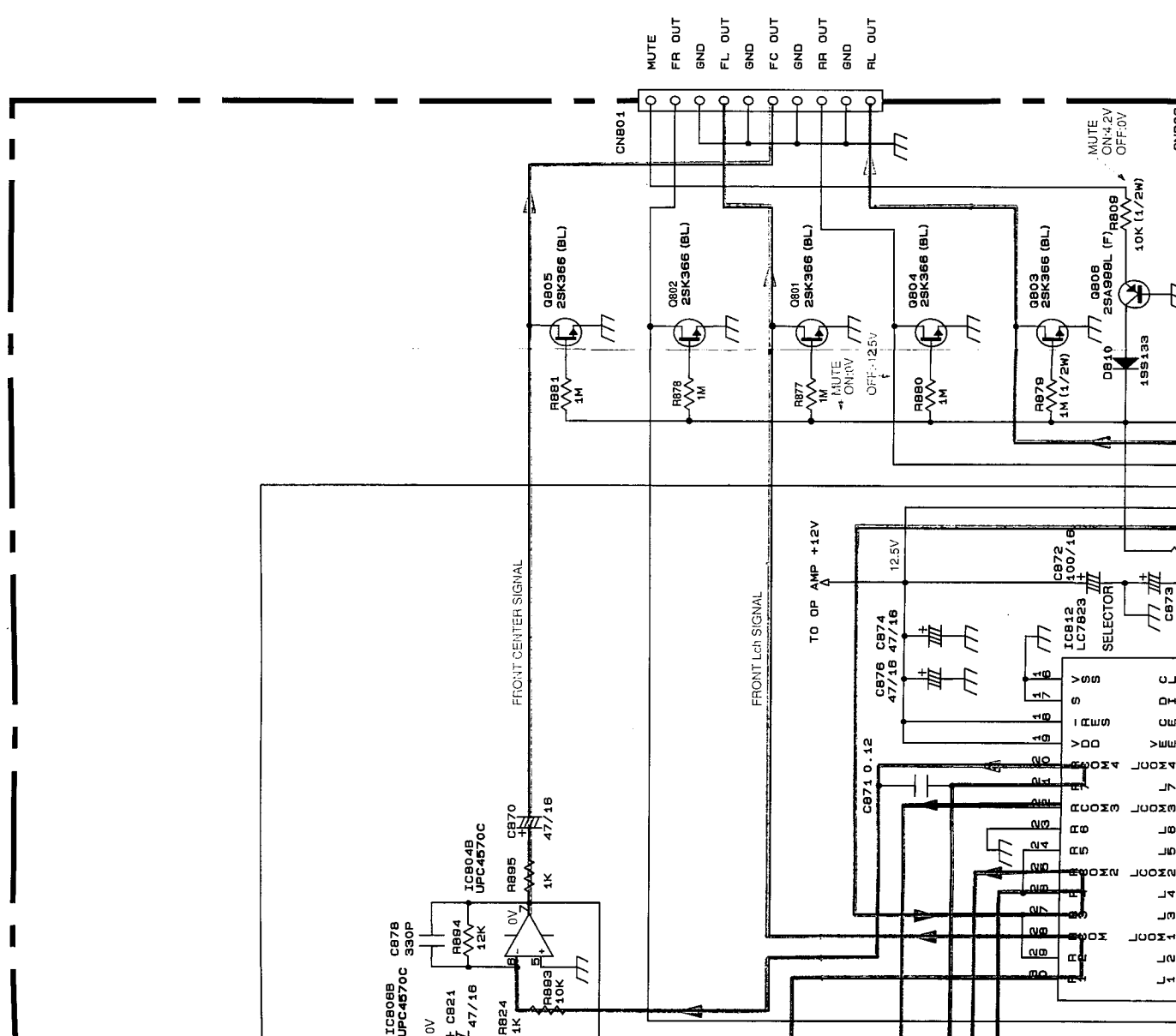
Page 46 SCHEMATIC DIAGRAM(11)
