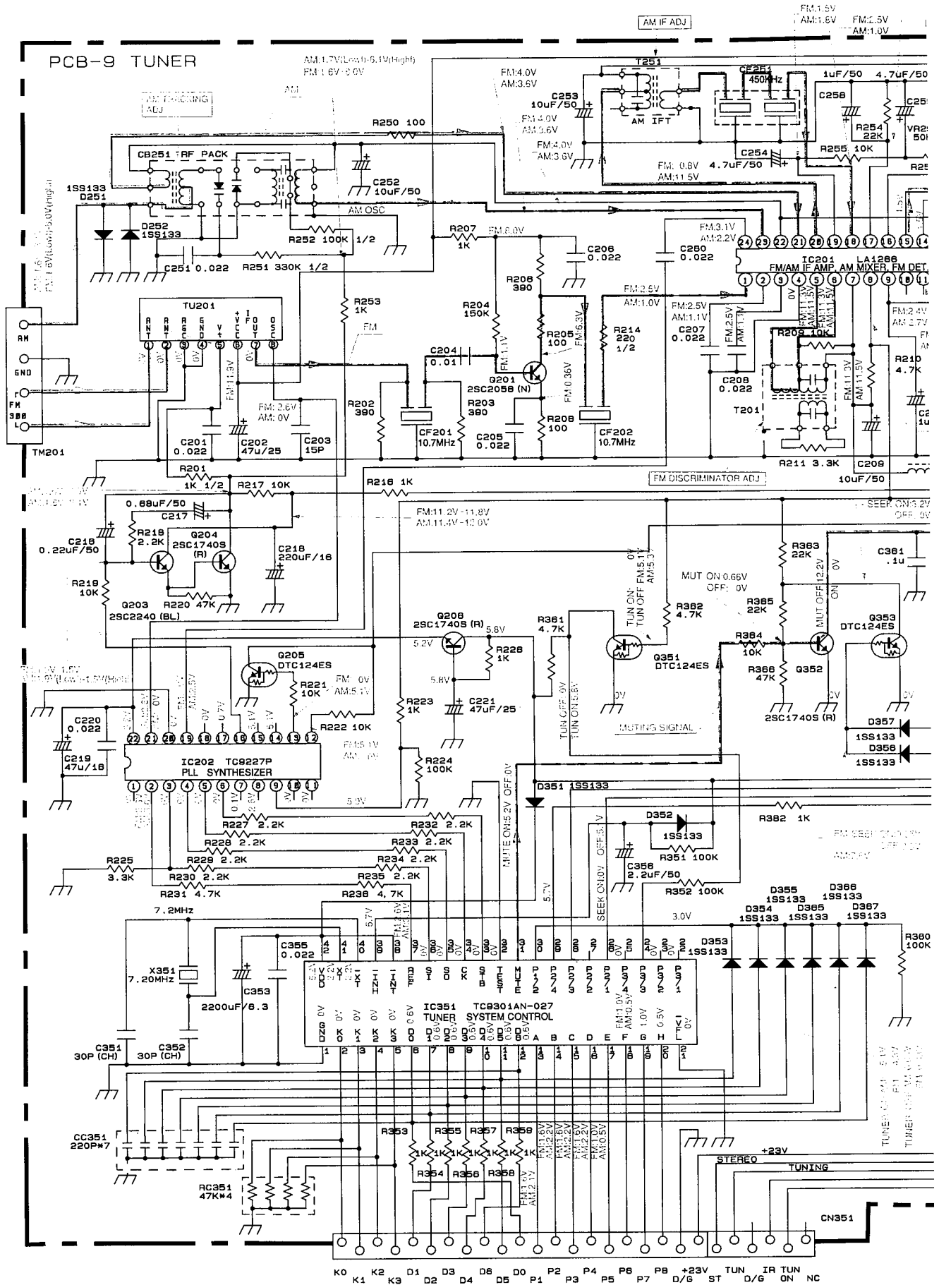
SCHEMATIC DIAGRAM(12)
