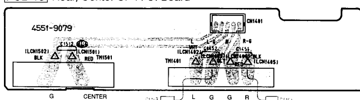
PCB-18 Rear, Center SP P. C. Board
