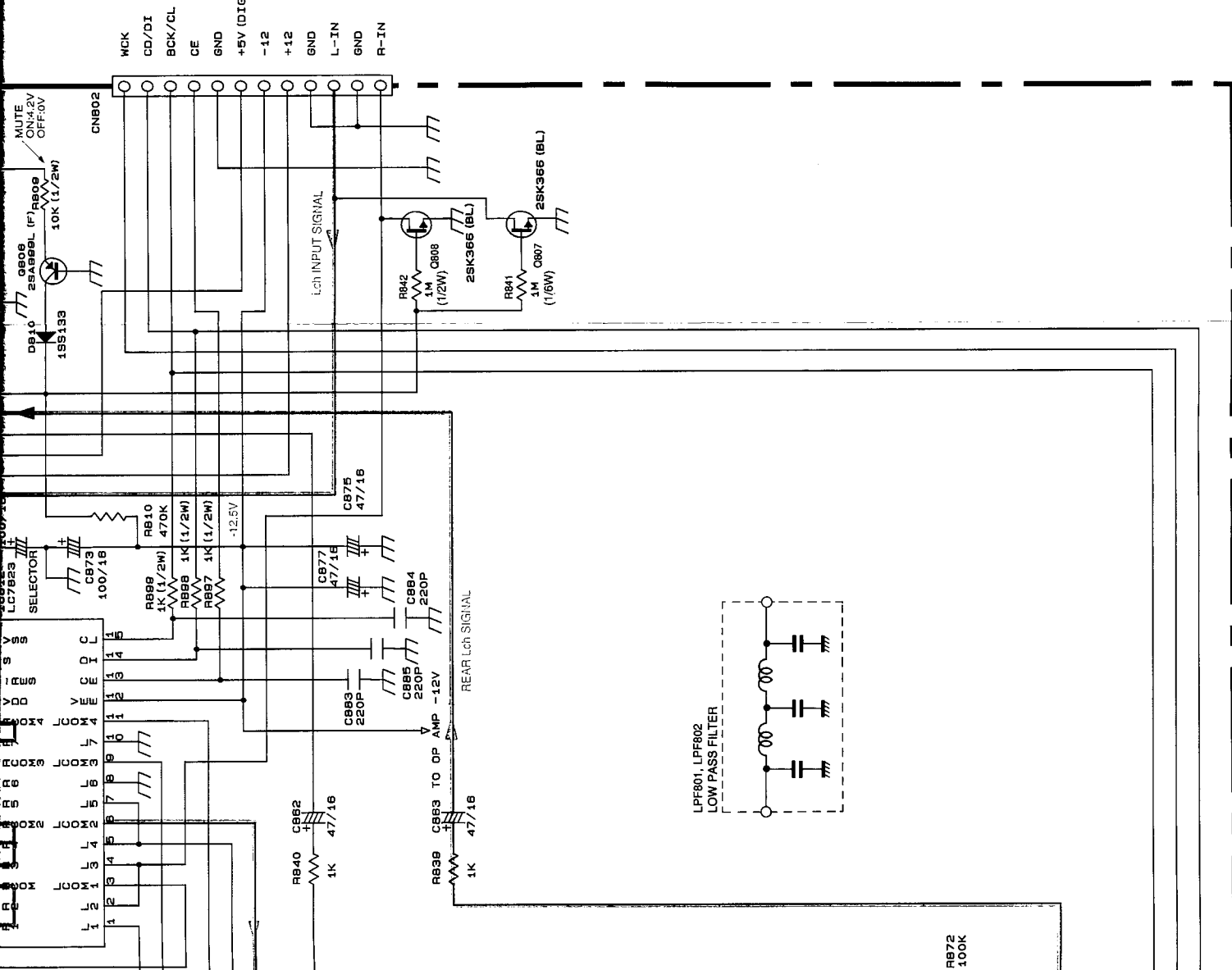
Page 46 SCHEMATIC DIAGRAM(11)
