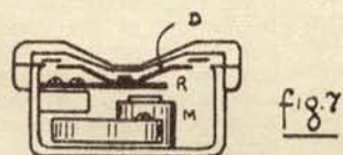
Section of the "Brown" telephone receiver
