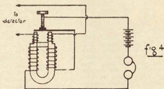
method of connecting up Brown relay
