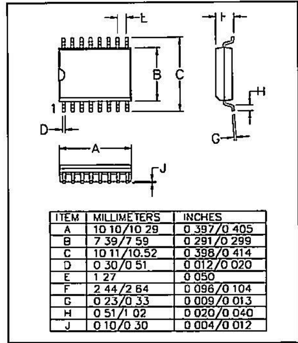
Figure 7 16-pin SO Wide package outline
