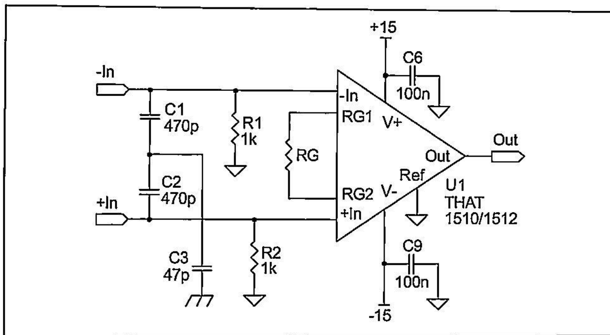
Figure 3 Basic 1510 / 1512 Circuit
