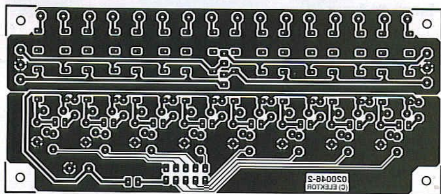
High-End Preamp — relay board 020046-2
