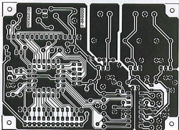
High-End Preamp — main board 020046-1
