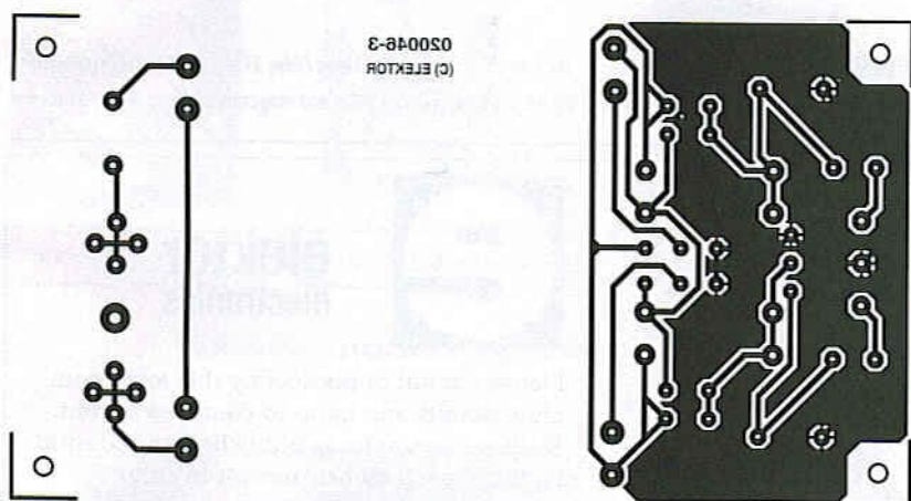
High-End Preamp — PSU board 020046-3
