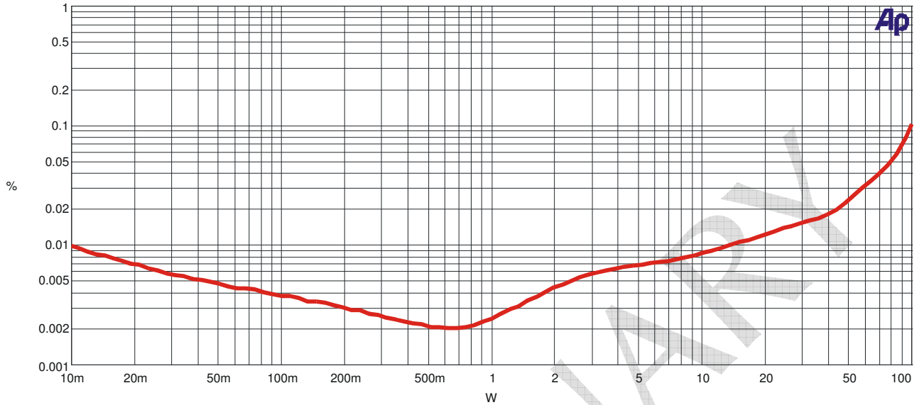
THD vs. Power (1kHz, 4Ω)
