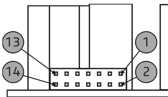
Fig1. Connector pinning UcD100™ (OEM version).
