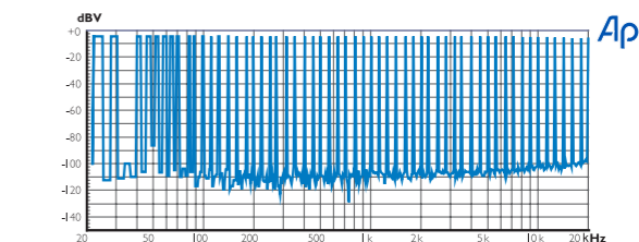
Fig. 13: Inter-modulation with multi-tone (6 tones per octave) input of MUETA prototype amplifier. Total RMS power is 5W.
