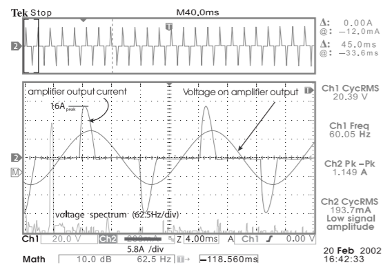
Fig. 14: Mueta prototype amplifier output voltage and -current when loaded with a rectifier.
