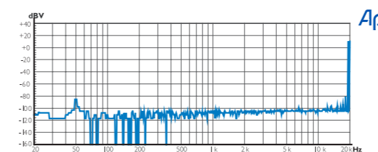
Fig. 12: Inter-modulation distortion measurement of MUETA prototype amplifier with 19kHz and 20kHz input at 5W.
