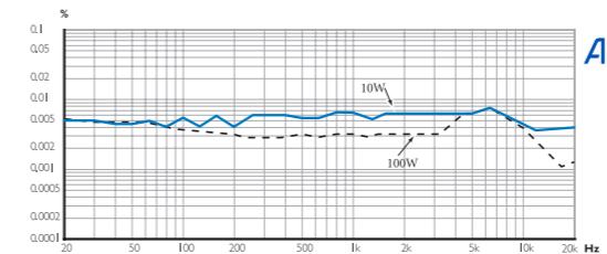
Fig. 10: THD (unweighted) versus frequency of MUETA prototype amplifier at 10W and 100W.
