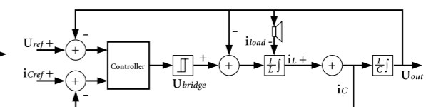
Fig. 8: Final block model of hysteresis amplifier with 2nd order output filter, capacitor current feedback and additional proportional feedback.
