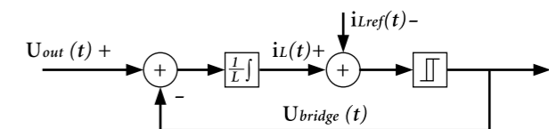
Fig. 6: Hysteresis controller with filtercoil integration and additional coil-current setpoint.
