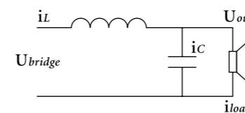
Fig. 5: Using the filtercoil as loop integrator in a hysteresis controller.
