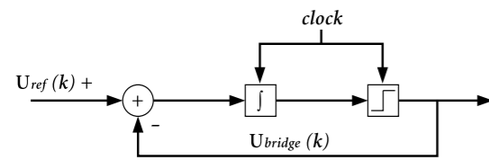
Fig. 1: Basic sampled \Sigma modulator circuit.
