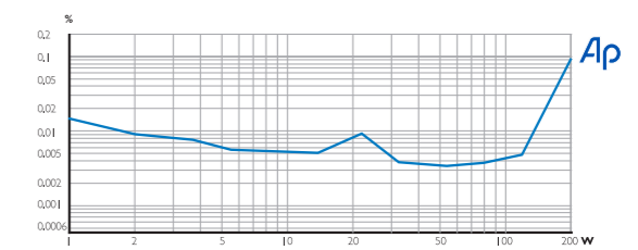
Fig. 11: THD (unweighted) versus power of MUETA prototype amplifier. Signal frequency is 1kHz.
