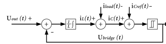
Fig. 7: Hysteresis controller with capacitor current feedback. Filter coil is used as loop integrator.
