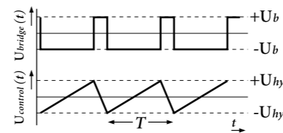
Fig. 3: Main signals in a hysteresis-controller circuit with DC input.
