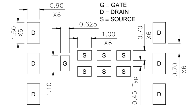
Figure A.18.3(b) L6-outline stencil design
