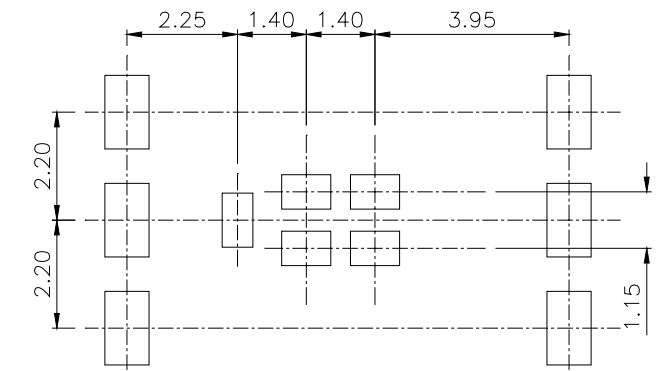
Figure A.17.3(a) L4-outline stencil design
