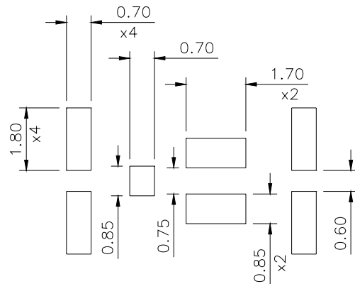
Figure A.8.3(b) MT-outline stencil design
