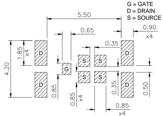
Figure A.16.2(b) M4-outline substrate/PCB layout
