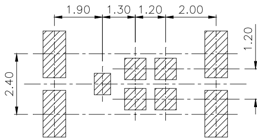
Figure A.16.2(a) M4-outline substrate/PCB layout
