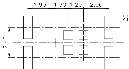
Figure A.16.3(a) M4-outline stencil design
