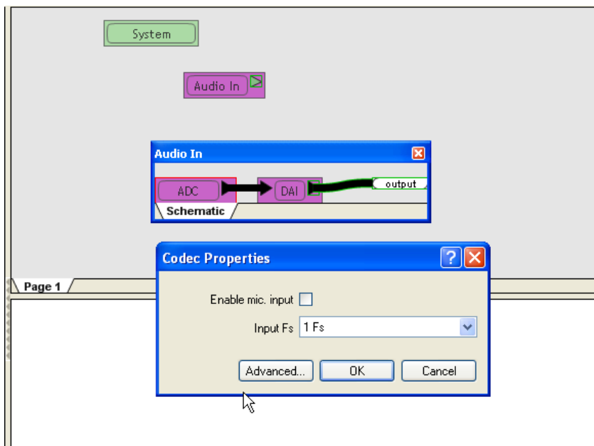
Figure 4-4. Audio In via 8 Channel ADC
