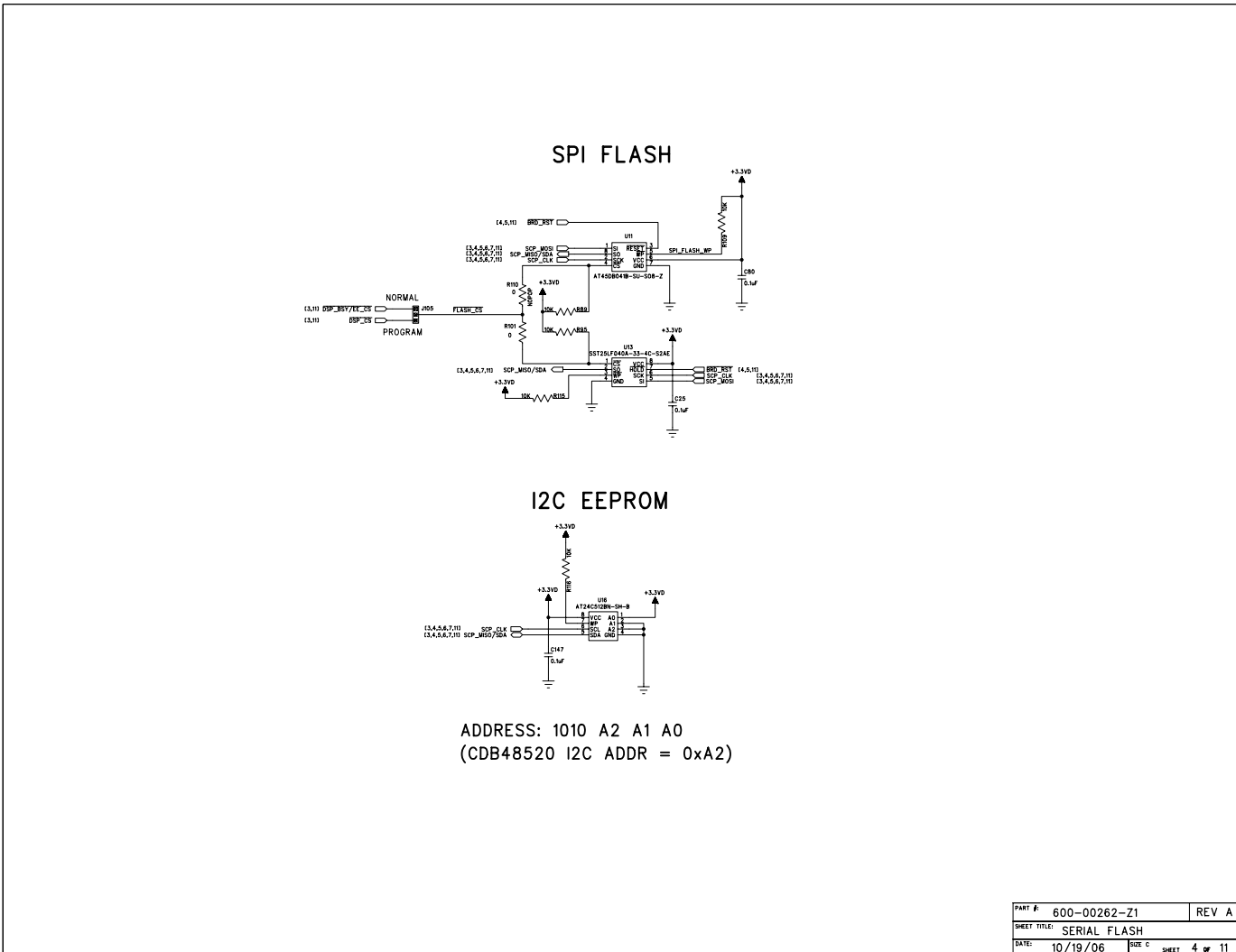
Figure A-4. Serial Flash Memory Schematic
