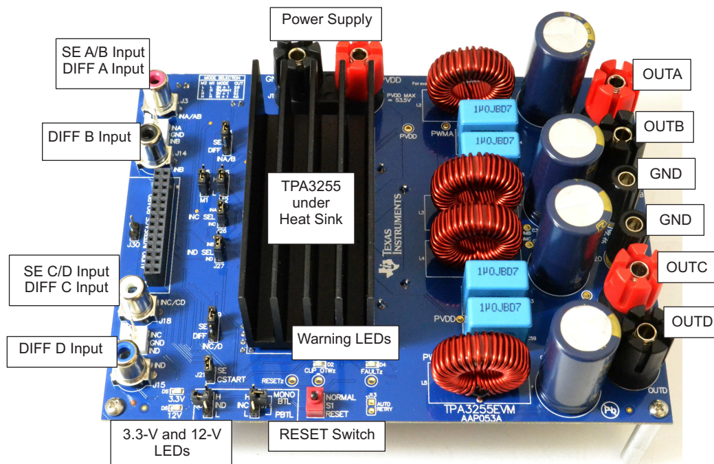
Figure 2. TPA3255EVM Connections
