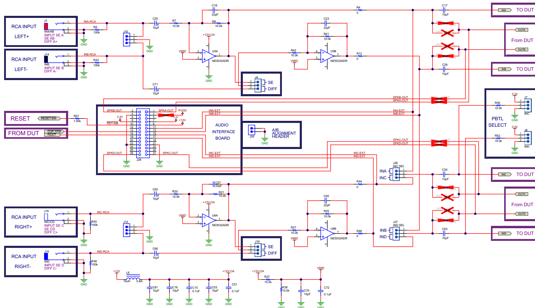
Figure 6. TPA3255EVM Schematic 1
