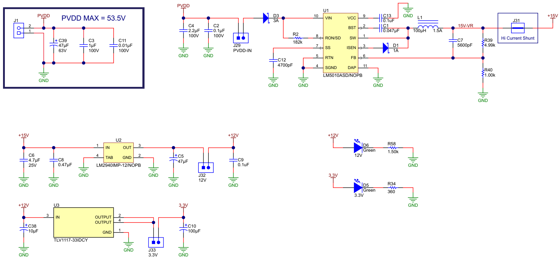
Figure 8. TPA3255EVM Schematic 3
