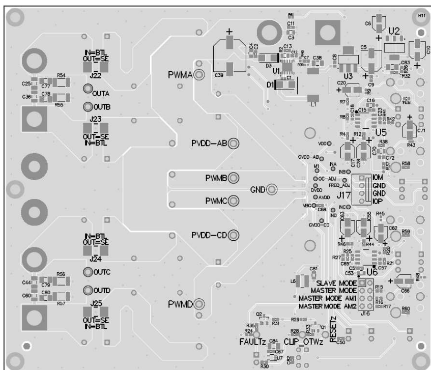
Figure 4. TPA3255EVM Bottom Composite Assembly
