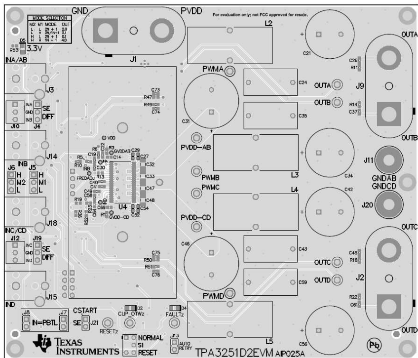
Figure 3. TPA3255EVM Top Composite Assembly
