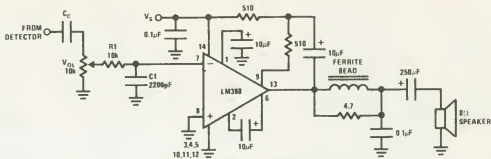
FIGURE 8. AM Radio Power Amplifier
