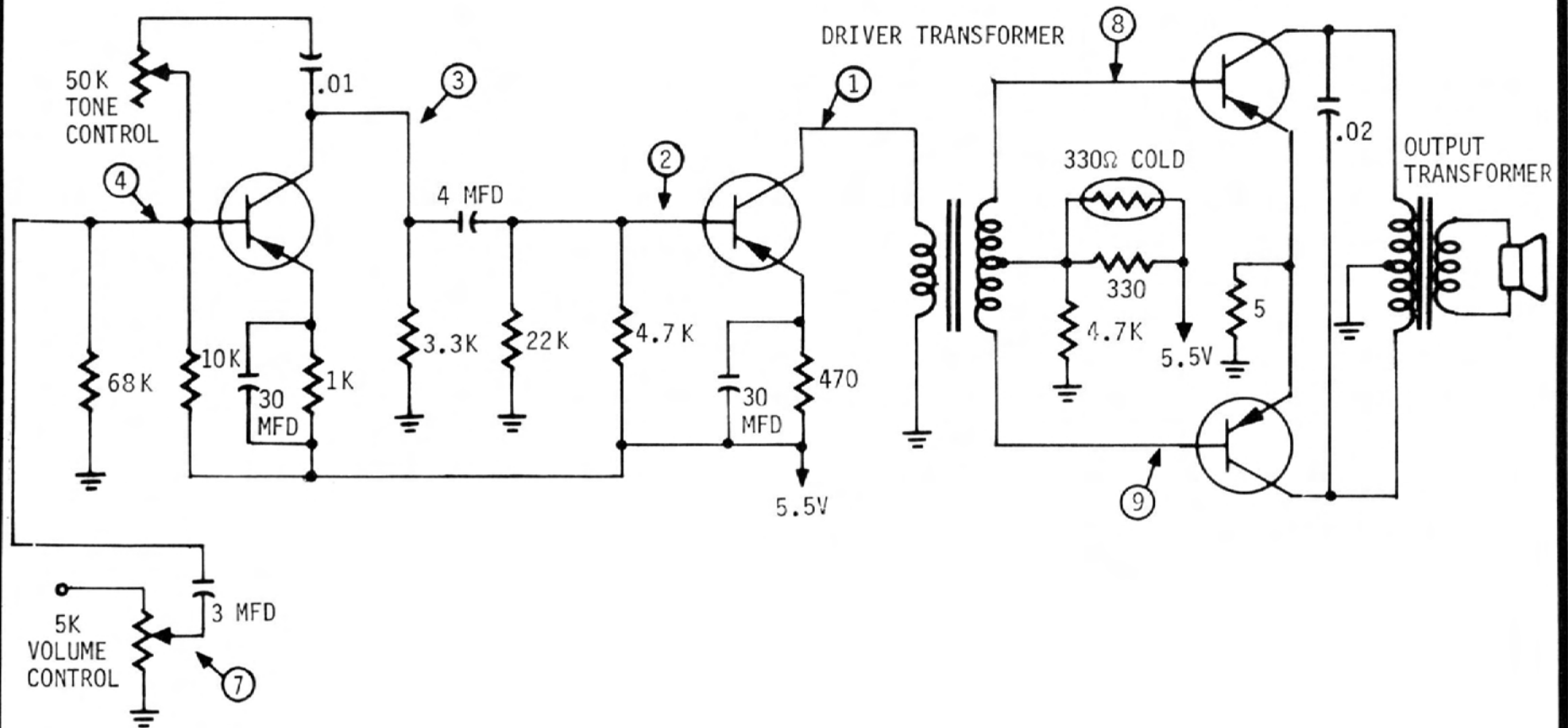
Fig. 4-2. A typical transformer-coupled audio amplifier with capacity-coupled pre-driver stage.
