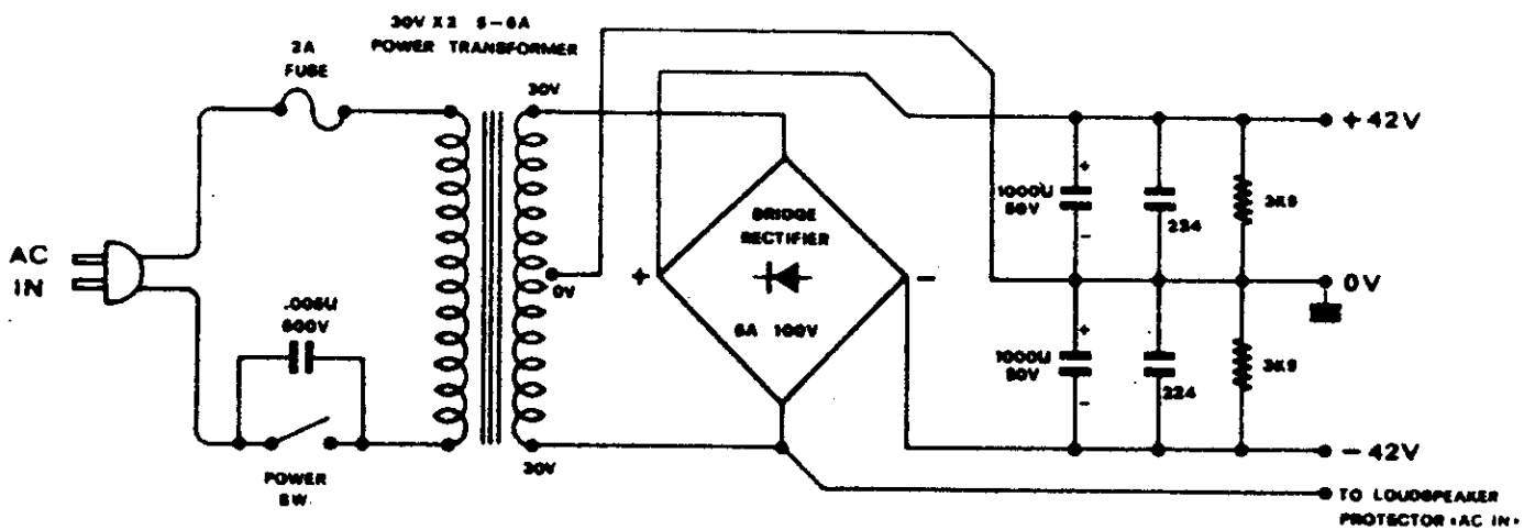
FIGURE 3 : THE POWER SUPPLY FOR TA-802.
