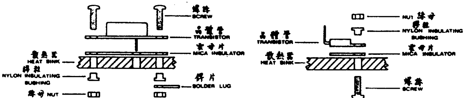
METHODS OF MOUNTING TO2 & TO3 TRANSISTORS ON HEAT SINK
