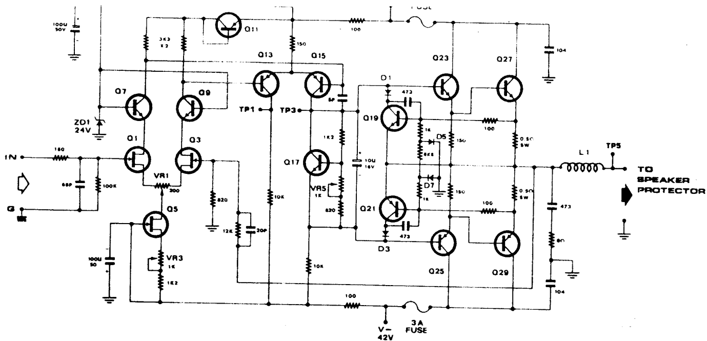
FIG 1:- CIRCUIT DIAGRAM OF THE LEFT CH. POWER AMP. UNIT.
