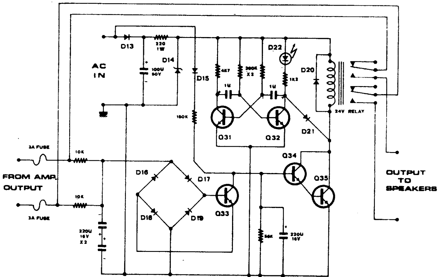
FIGURE 2 : CIRCUIT DIAGRAM OF THE TA-802 LOUDSPEAKER PROTECTOR UNIT.
