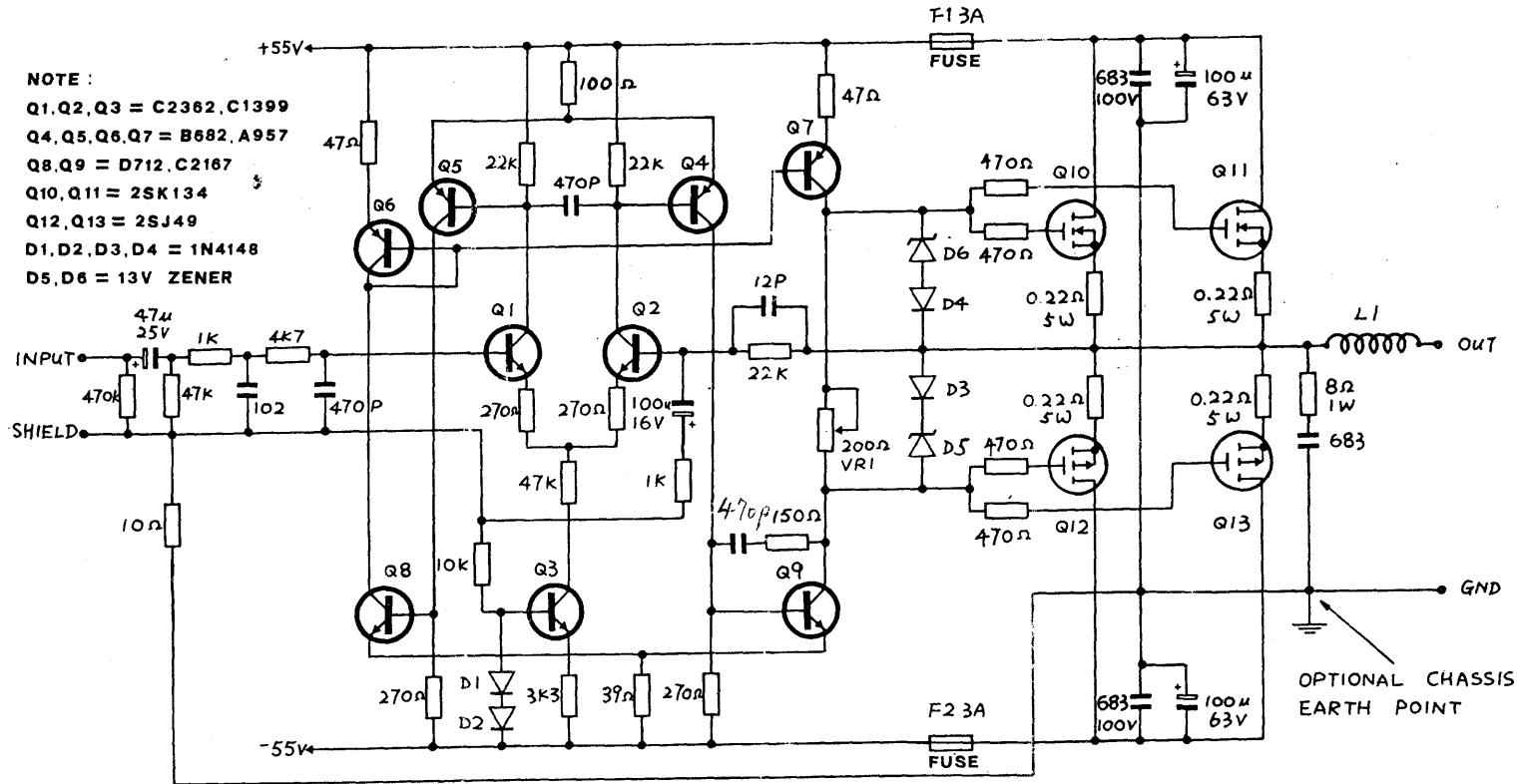
(FIG. 1) CIRCUIT DIAGRAM OF THE TA-477 MOSFET POWER AMPLIFIER.
