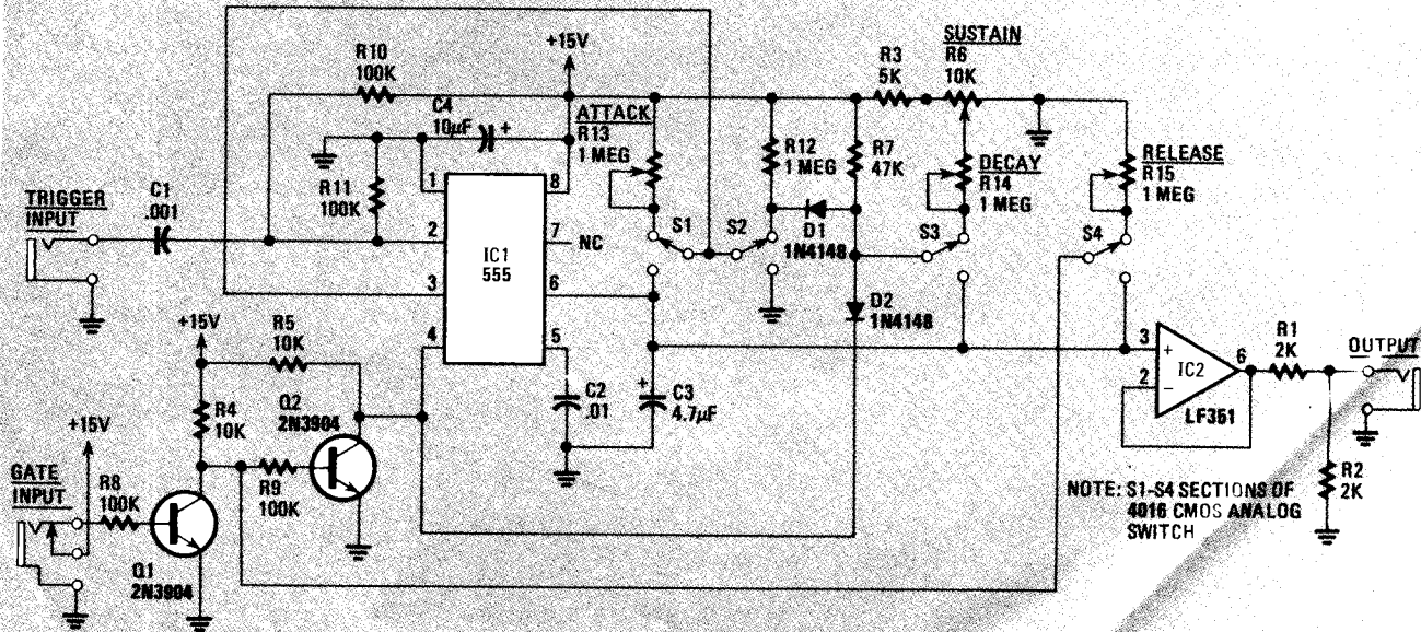
FIG. 5—THIS ADSR ENVELOPE GENERATOR circuit provides you with complete control over the attack time, decay time, sustain level, and release time.
