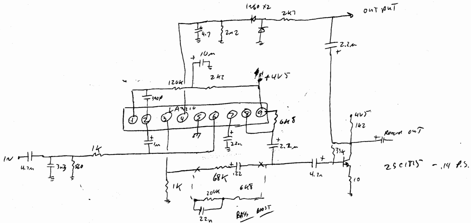
m950 Record Circuit - Pre Amp for ALC.
