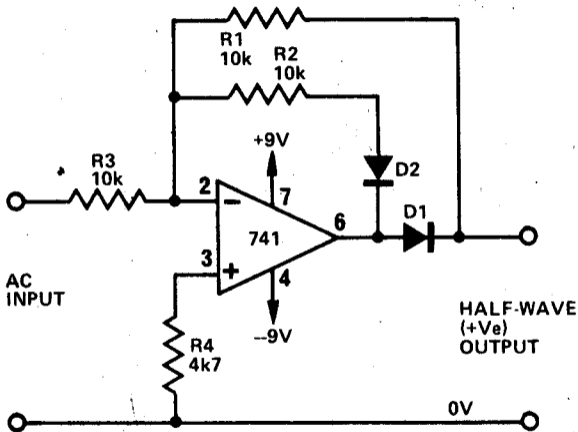
Fig. 26a Precision unity-gain half-wave rectifier.
