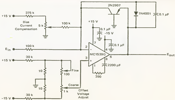
Fig. 30-1. Logarithmic amplifier using an MC1539G op amp (M).
