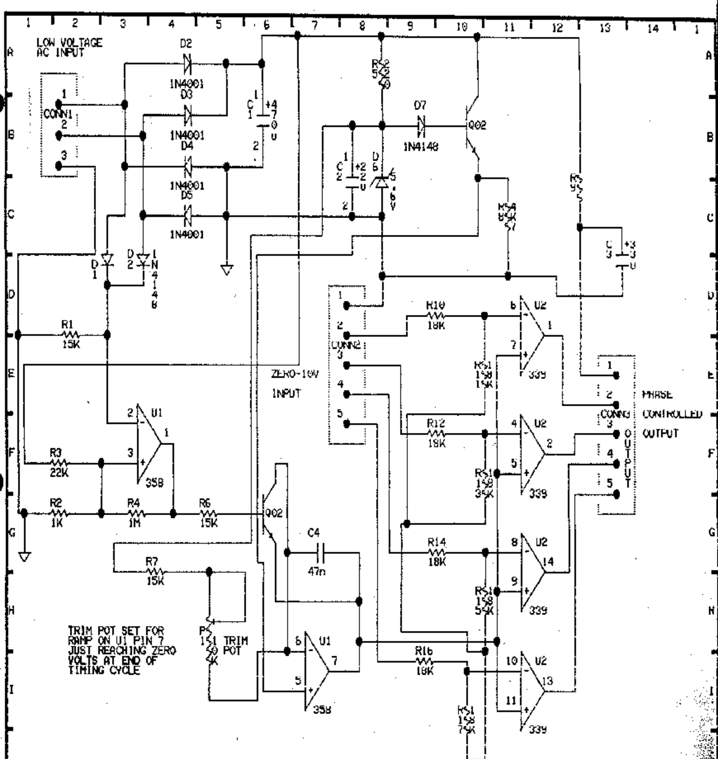
Interface to convert 0-10V Dimmer Signal to phase controlled signal for disco type triac power packs.
