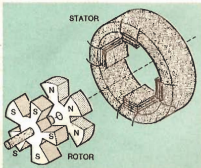
FIG. 1—A SIMPLIFIED DIAGRAM shows how stepper motors are built.
