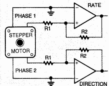
FIG. 11—TO USE A STEPPER as a shaft encoder, the output signals must be converted to square waves with a pair of voltage comparators.
